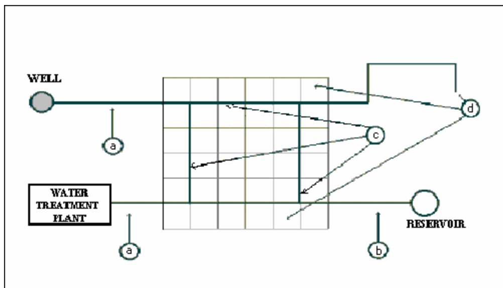
Figure 3. Sampling Sites in Mixed Distribution Systems
